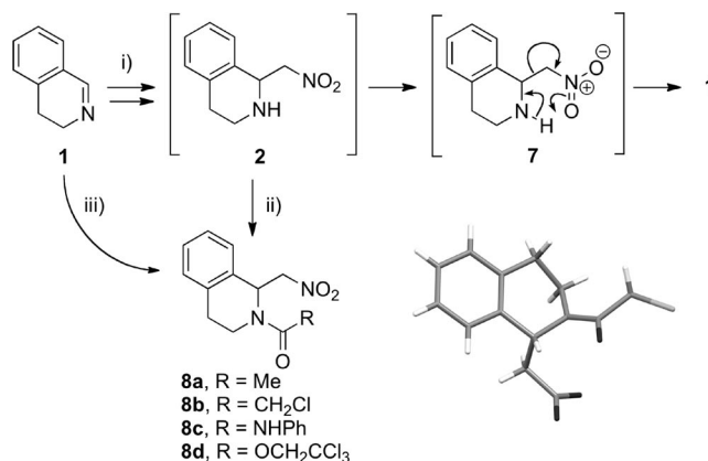
Scheme 2. Decomposition, and acylation, of unstable \beta -nitroamine 2 . Reagents and conditions: i) nitromethane, triethylamine; ii) for 8a : acetyl chloride, for 8b : chloroacetyl chloride and 2,2,6,6-tetramethylpiperidine; iii) One-pot protocol: nitromethane, acylating agent (1.1 equiv.), triethylamine (1.1 equiv.), 45 °C, 2 h. Inset: crystal structure for 8b .
