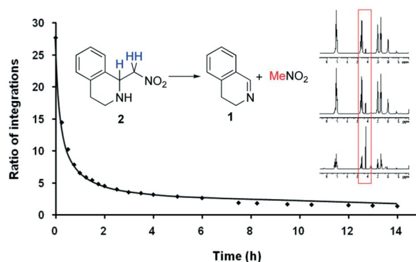
Figure 1. Kinetic study on the instability of \beta -nitroamine 2 and the corresponding 1 H NMR spectra at the following times: (i) 0 min (top); (ii) 15 min (middle) and (iii) 14 h (bottom). The ratio calculated is the integral of the signals for the three protons marked blue in the nitroamine ( 2 ) vs. the signals for the protons marked red for the nitromethane produced by the decomposition reaction (linear scale of NMR spectra in inset is 0 to 8 ppm).
