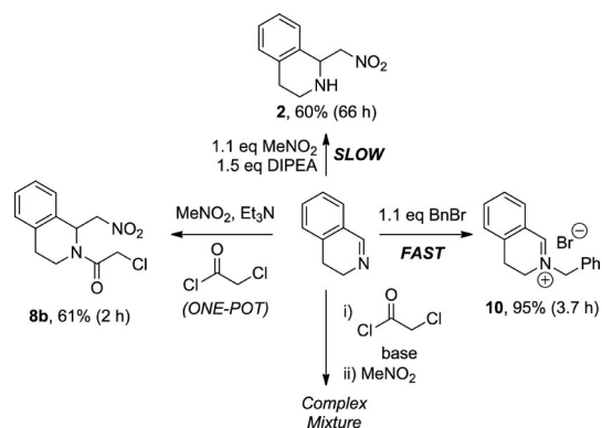
Scheme 4. Investigations into the mechanism of the quenched aza-Henry reaction of dihydroisoquinoline.
