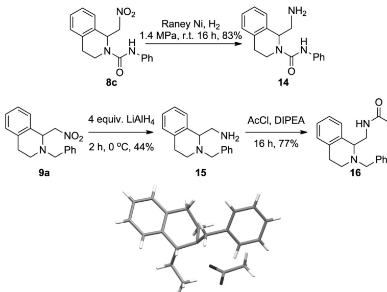
Scheme 7. Reductions of nitro compounds 8c and 9a , and X-ray crystal structure of 15·OAc .
