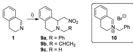
Scheme 3. Aza-Henry reaction with alkylation. Reagents and conditions: i) as for one-pot procedure, Scheme 2; 9c synthesized by a two-step process.
