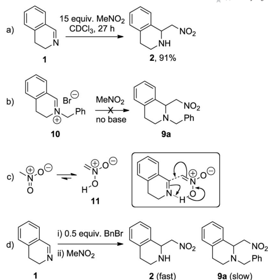
Scheme 5. Experiments towards understanding the mechanism of the aza-Henry reaction between 3,4-DHIQ and nitromethane.
