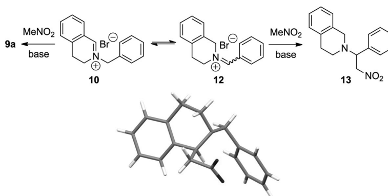
Scheme 6. Potential tautomerism in 10 , and crystal structure of the isolated product 9a .
