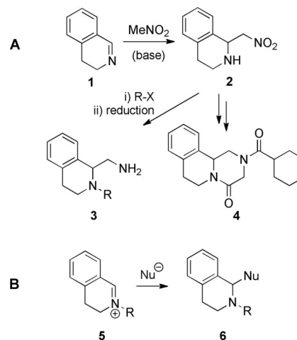
Scheme 1. The aza-Henry reaction with 3,4-DHIQ (A) in the synthesis of chiral diamines ( 3 ) and praziquantel ( 4 ), and (B) the comparison with traditional Reissert-type reactions.
